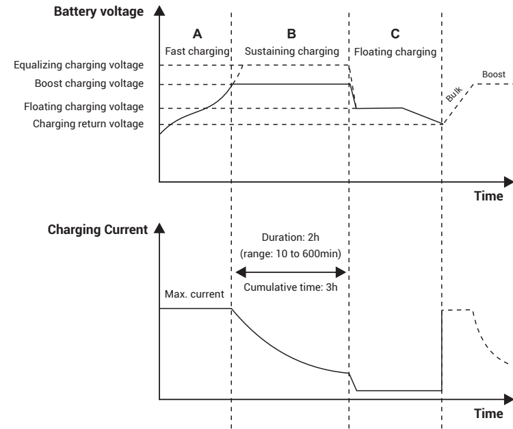
Fig. 1-5 Battery charging stages diagram
