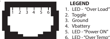
Fig. 3.2 Remote Control RC-15A - Pinout of Modular Jack RJ-12 / RJ-25
